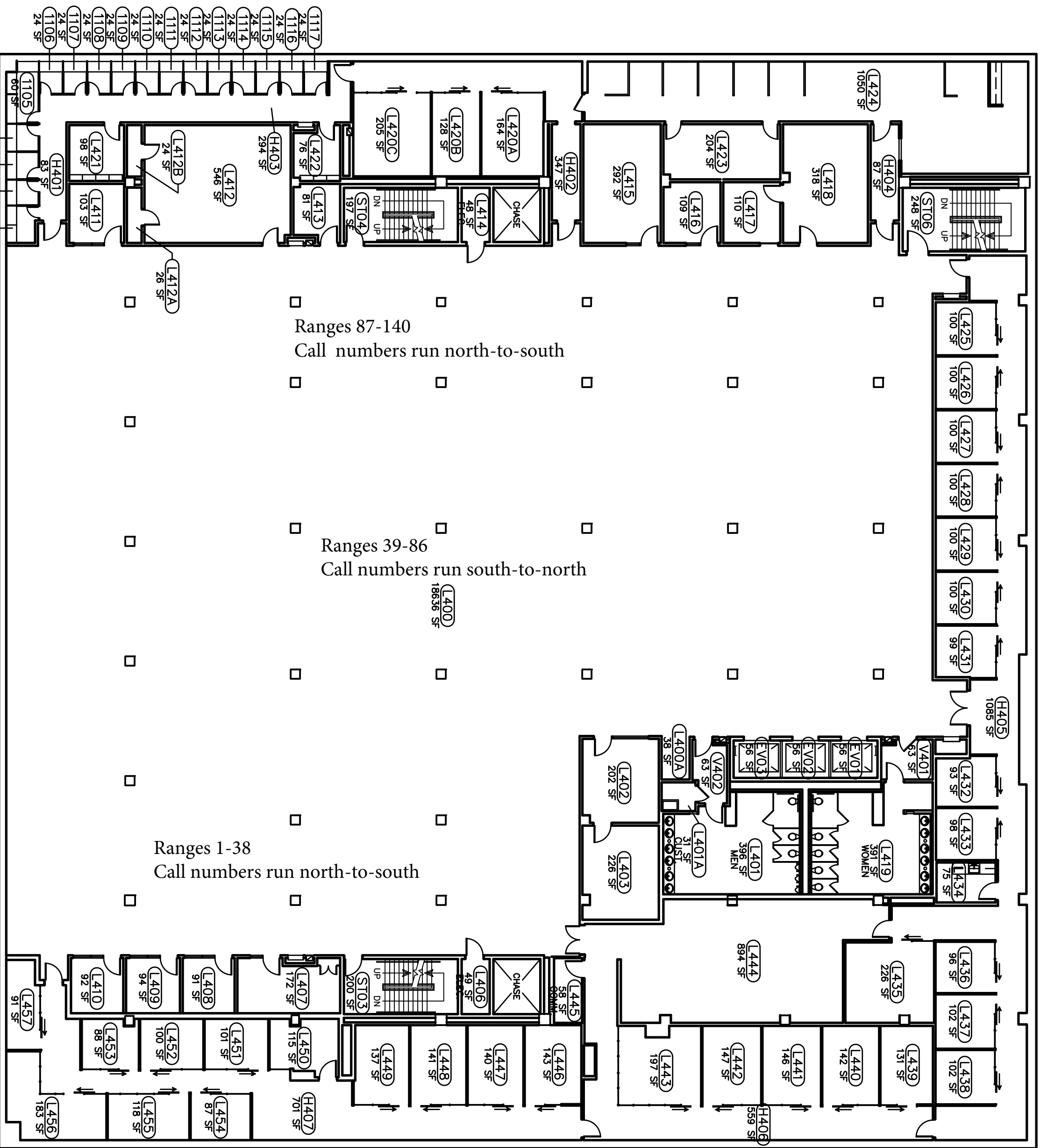
(LEVEL 4) SUB-BASEMENT ONE FLOOR PLAN - 103 SCALE: 1/16" = 1'-0"
